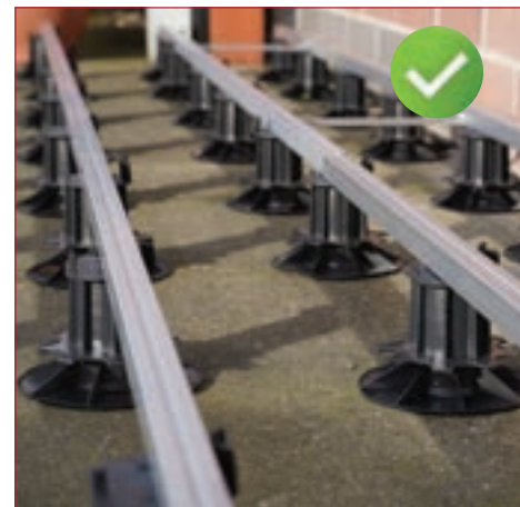
A structurally sound sub frame must be installed ensuring there is no movement prior to fixing boards to the joists. A 1.66% (1:60) fall to allow water to drain and a minimum 100mm free air space between the boards and the ground beneath to allow sufficient airflow to prevent the build up of moisture is essential.
